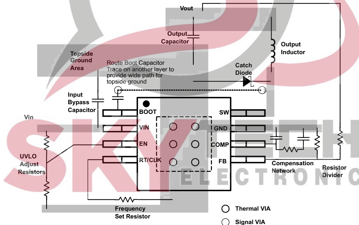
Figure 52. PCB Layout Example
